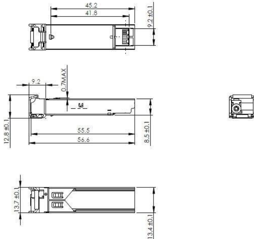
Mechanical Drawing
